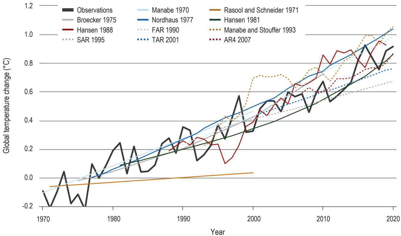
IPCC, Climate Change 2021, The Physical Science Basis, Figure 1.9
