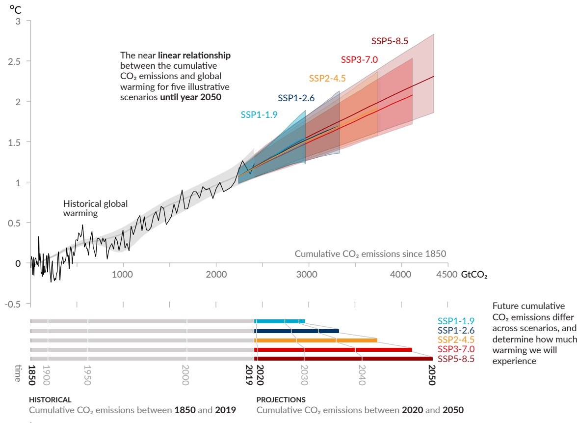
Figure SPM.10: Near-linear relationship between cumulative CO 2 emissions and the increase in global
