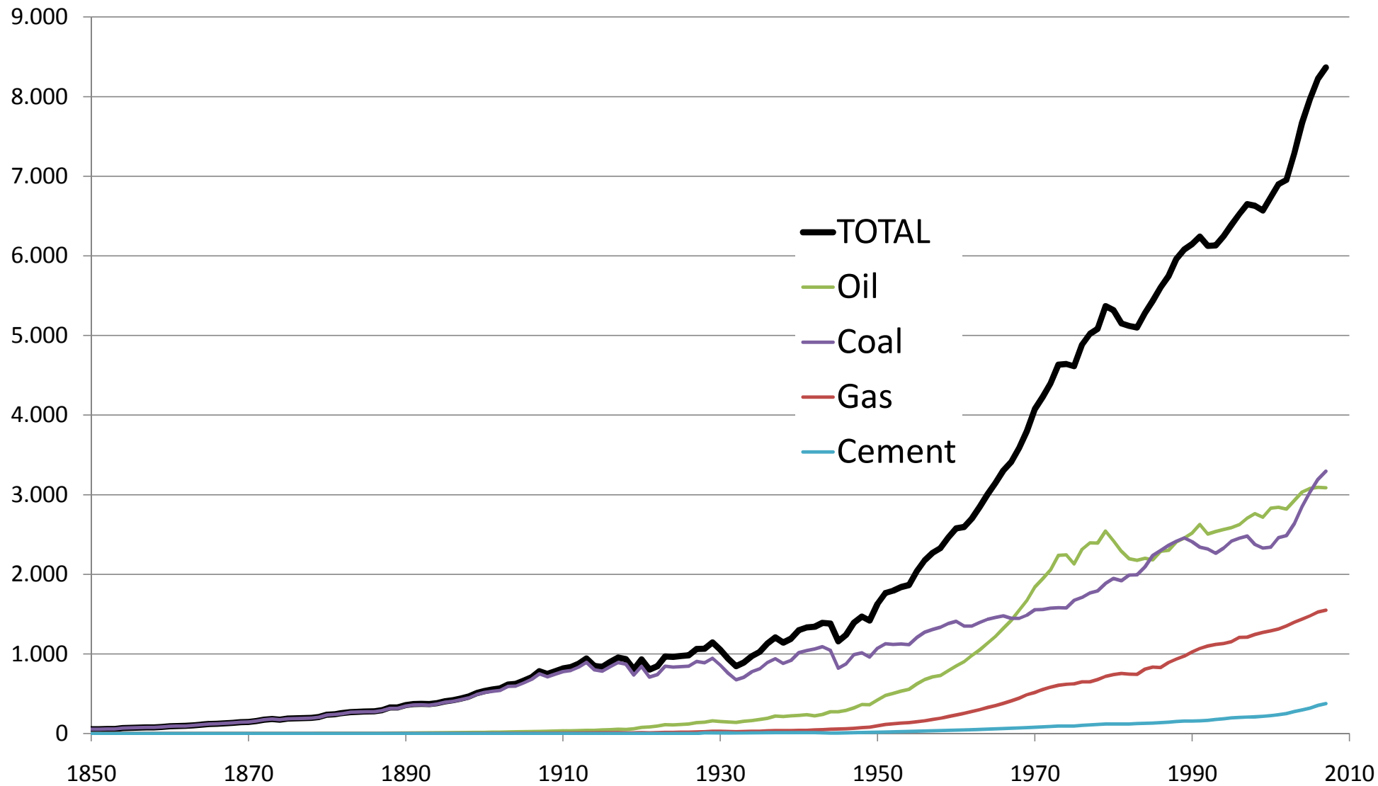
Global Fossil-Fuel Carbon Emissions (millions tons - http://cdiac.ornl.gov/ )
