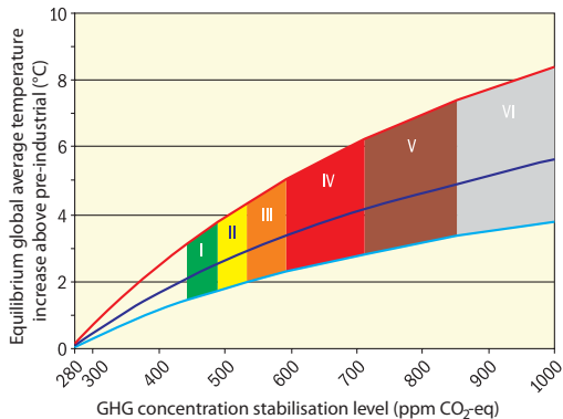
Figure 5.10: Left: CO 2 emissions scenarios from global successful thrive for clean energies, I, to business-as-usual, VI. Right: Corresponding long term atmospheric level of greenhouse gases and global average temperature increase above pre-industrial. Sources: IPCC.
