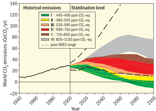
Figure 5.10: Left: CO 2 emissions scenarios from global successful thrive for clean energies, I, to business-as-usual, VI. Right: Corresponding long term atmospheric level of greenhouse gases and global average temperature increase above pre-industrial. Sources: IPCC.
