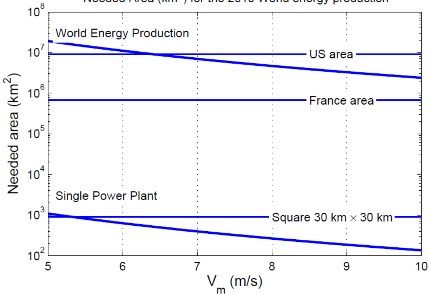
Needed Area ( \text{km}^2 ) for the 2010 World energy production
