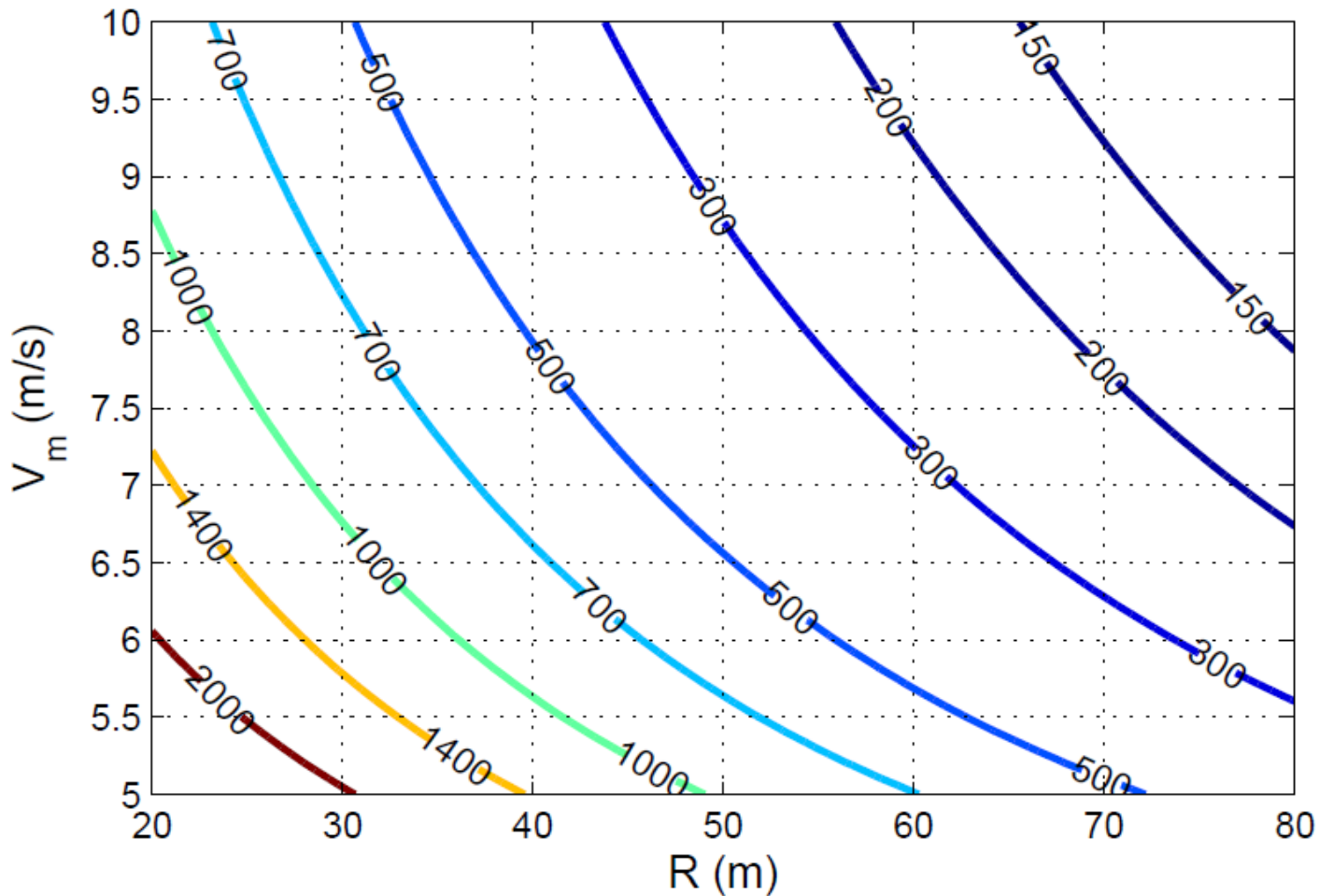
Needed Length (km) for one 1 GW Power Plant
