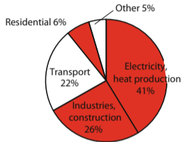
CO 2 break-up
