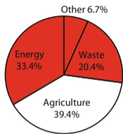
CH 4 break-up
