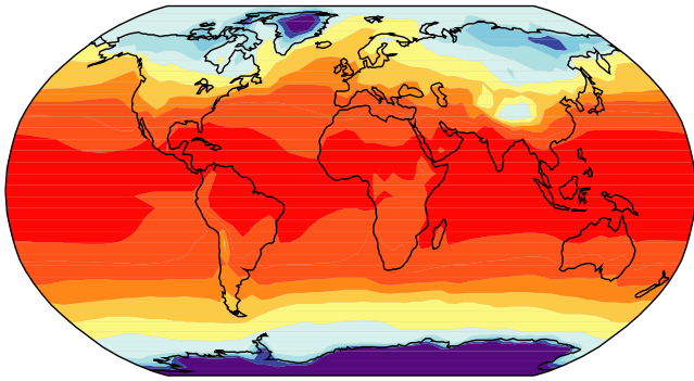
Observations 1980 -1999
