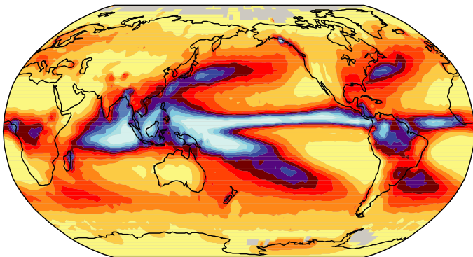
Observations 1980 -1999
