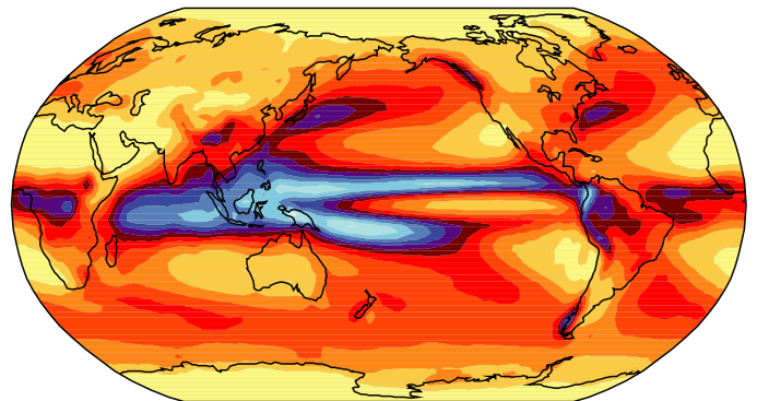
Average 23 Models
