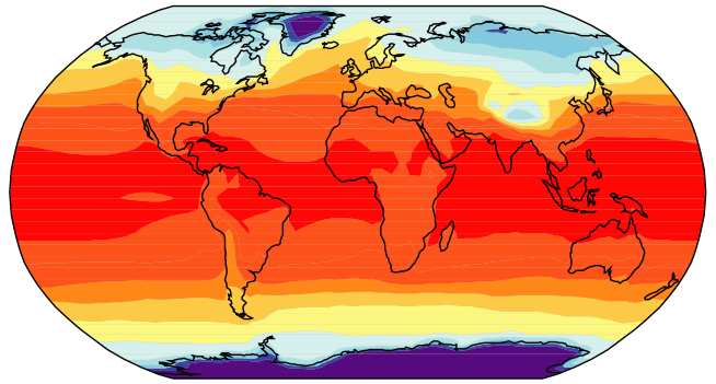
Average 23 Models
